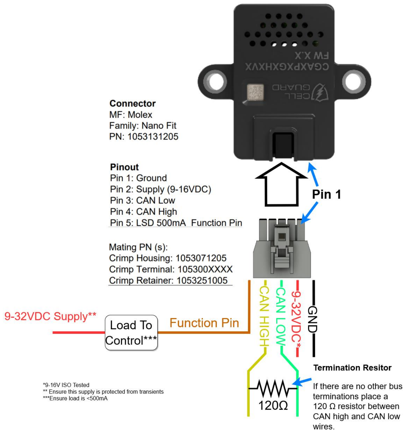
FIGURE 3 WIRING EXAMPLE
