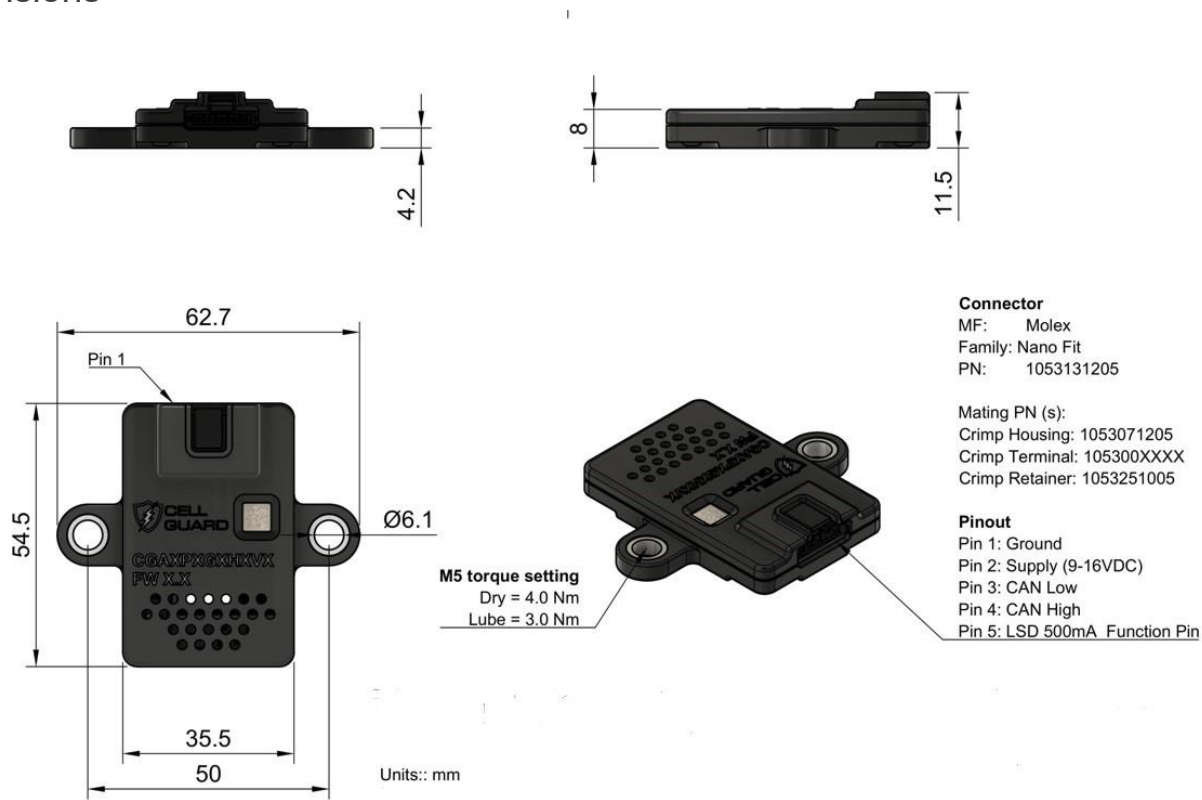
FIGURE 4 SENSOR DIMENSIONS
